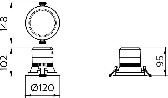
Dimensional drawing
