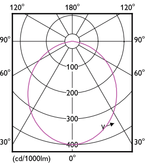
Light Distribution Diagram - DN027B LED6/NW D90 RD
