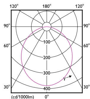
Light Distribution Diagram - DN027B LED3/NW D100 RD
