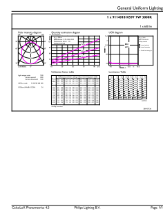
General uniform lighting - DN027B LED6/WW D100 RD
