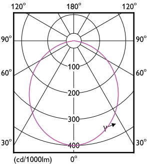
Light Distribution Diagram - DN027B LED6/NW D125 RD
