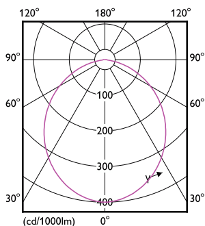
Light Distribution Diagram - DN027B LED6/NW D125 RD
