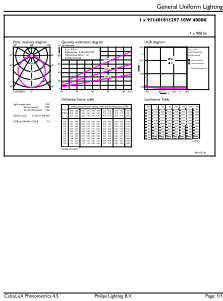
General uniform lighting - DN027B LED9/NW D125 RD
