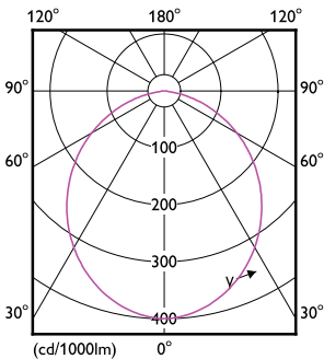
Light Distribution Diagram - DN027B LED6/NW D150 RD
