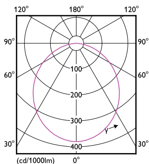
Light Distribution Diagram - DN027B LED12/WW D150 RD
