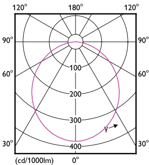
Light Distribution Diagram - DN027B LED12/NW D175 RD
