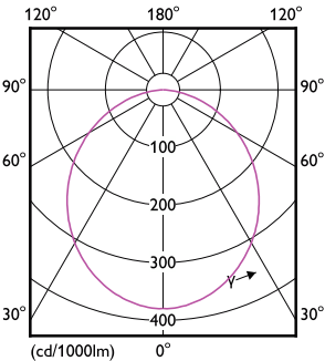
Light Distribution Diagram - DN027B LED12/CW D175 RD
