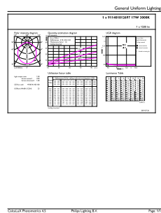
General uniform lighting - DN027B LED15/WW D175 RD
