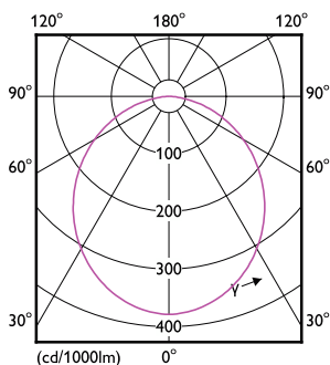
Light Distribution Diagram - DN027B LED15/WW D200 RD
