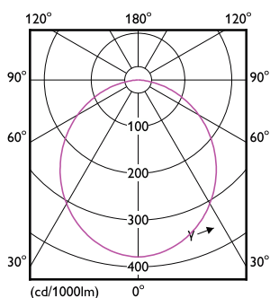
Light Distribution Diagram - DN027B LED15/CW D200 RD
