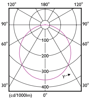
Light Distribution Diagram - DN027B LED3/NW L100 SQ
