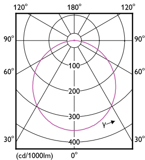
Light Distribution Diagram - DN027B LED3/NW L100 SQ
