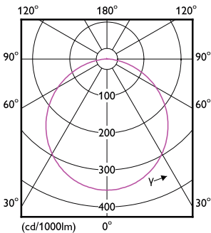
Light Distribution Diagram - DN027B LED6/NW L100 SQ
