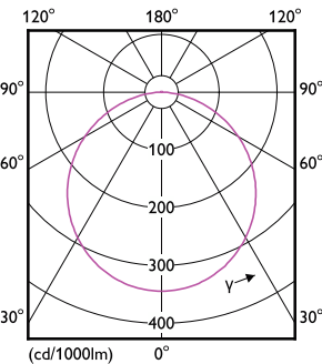
Light Distribution Diagram - DN027B LED6/CW L150 SQ
