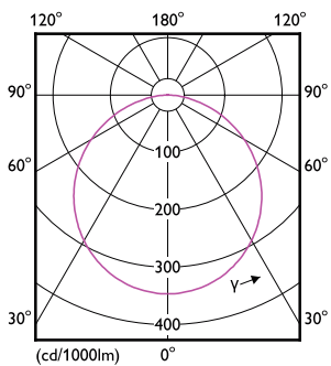
Downlight DN027B LED12 NW L150 SQ
