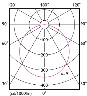
Light Distribution Diagram - DN027B LED12/CW L150 SQ
