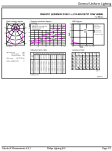
General uniform lighting - DN027C LED9/NW D150
