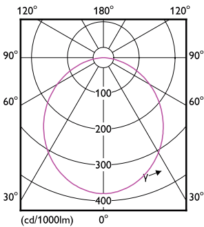
Light Distribution Diagram - DN027C LED12/WW D175
