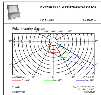
OFPC1_BVP650T251xLED120-4S740OFA52
