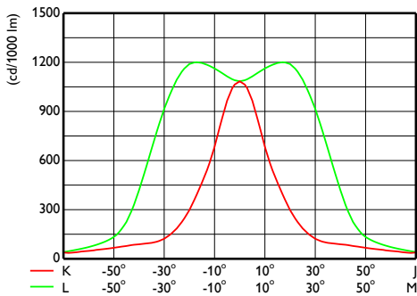
OFCS1_BVP651T251xLED450-4S740S
