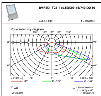
OFPC1_BVP651T251xLED500-4S740DX10
