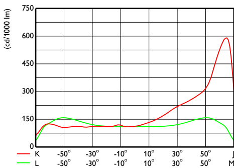
OFCS1_BVP651T251xLED500-4S740DX50
