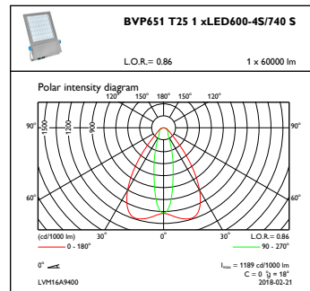
OFPC1_BVP651T251xLED600-4S740S
