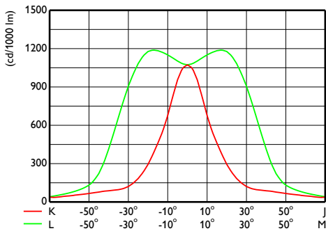
OFCS1_BVP651T251xLED600-4S740S
