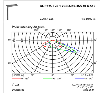
OFPC1_BGP625T251xLED240-4S740DX10
