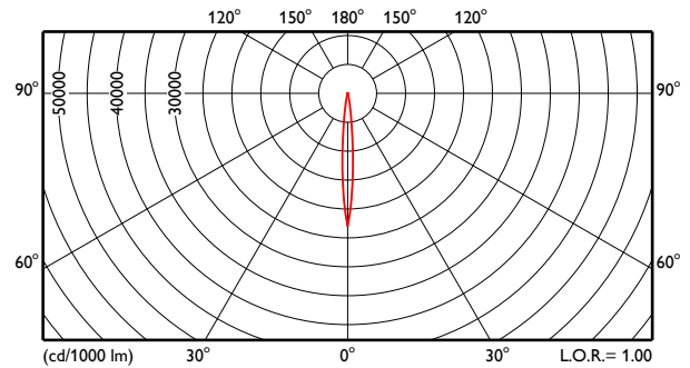
OFCS1_BCP48336xLED-HBRGBMW-270010
