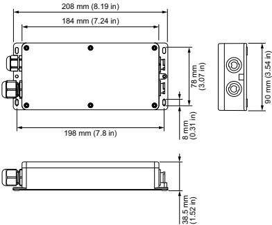
ZCX401 CTRL MOD ETH 24V 2xOUT IP66
