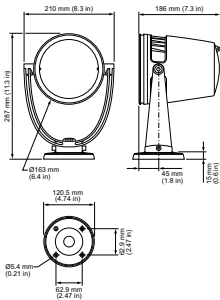
BCP463 G2 19xLED-HB/2700 GR
