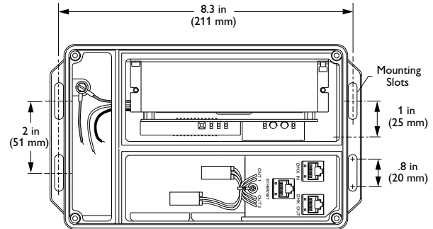
Power/data supply units ZCX400
