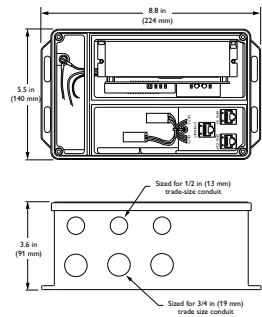
Power/data supply units ZCX400
