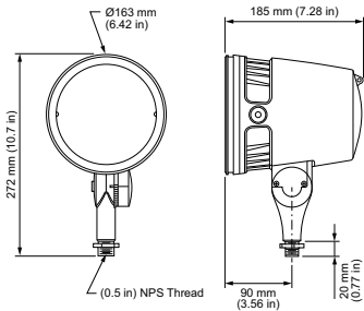
BCP463 G2 19xLED-HB/3500 HMA GR
