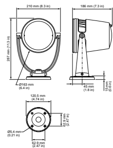
BCP462 G2 19xLED-HB/RGBMW WH
