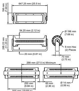
DCP773 36xLED-HB/2700K
