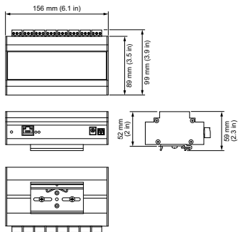
Power/data supply units ZCX400
