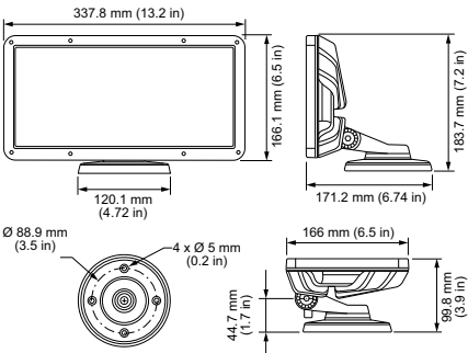
BCP484 36xLED-HB/RGBW FTA 100-277V BK
