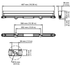
BCS425 RGBW FR ETH L457 PP19
