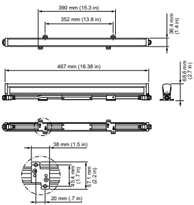
BCS425 RGBW CL ETH L457 PP19
