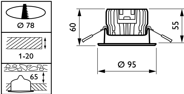
CoreLine RS140B/RS141B
