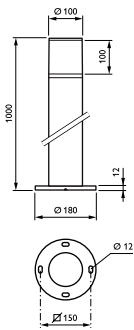
CoreLine Bollard BCP155
