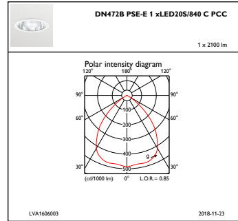
IFPC1_DN472BPSE-E1xLED20S840CPCC
