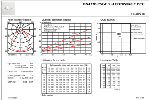
IFGU1_DN472BPSE-E1xLED20S840CPCC
