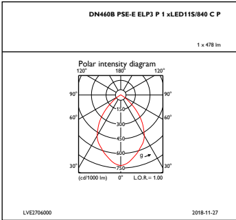
IFPC1_DN460BPSE-EELP3P1xLED11S840CP
