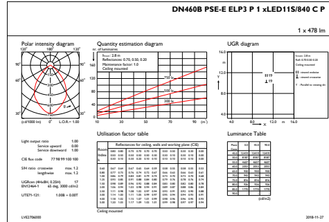
IFGU1_DN460BPSE-EELP3P1xLED11S840CP
