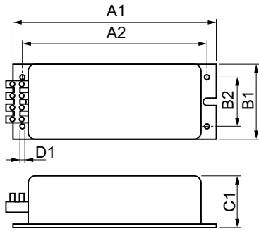
BSX 91 H96 220-240V 50Hz CW-149/67
