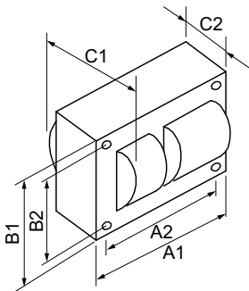
MH BAL 175W M57 120/277/347V KIT
