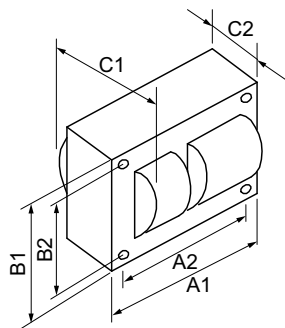
HPS BAL 150W S55 120/208/240V C&C
