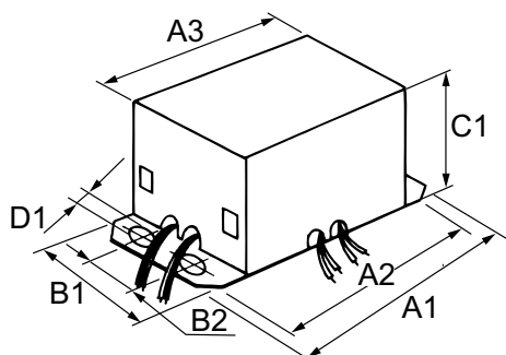
MH BAL 400W M59/H33 QUAD ENCAP
