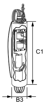
HPS BAL 100W S54 208V POSTLINE
