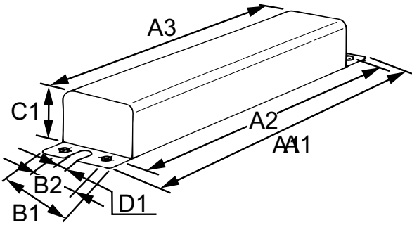
MH BAL 70W M98/143 120/347V FCAN
