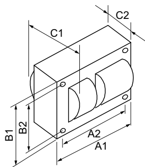
HPS BAL 100W (EURO LAMP) 127/220/240 C&C
